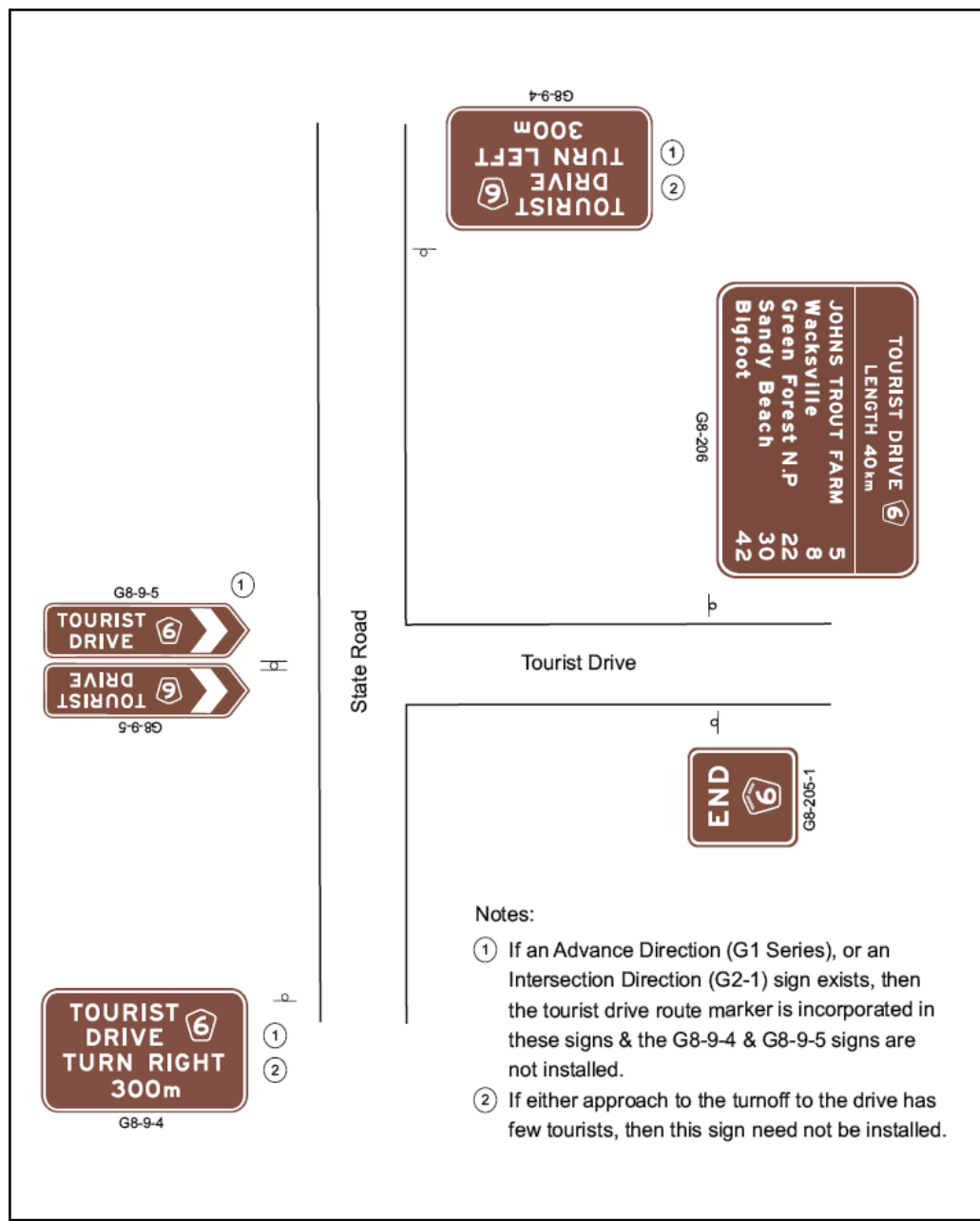
Figure 3.49 Typical arrangement of Tourist Signs at the start / finish of a Regional Tourist Drive that has no Major Tourist Focal Point
