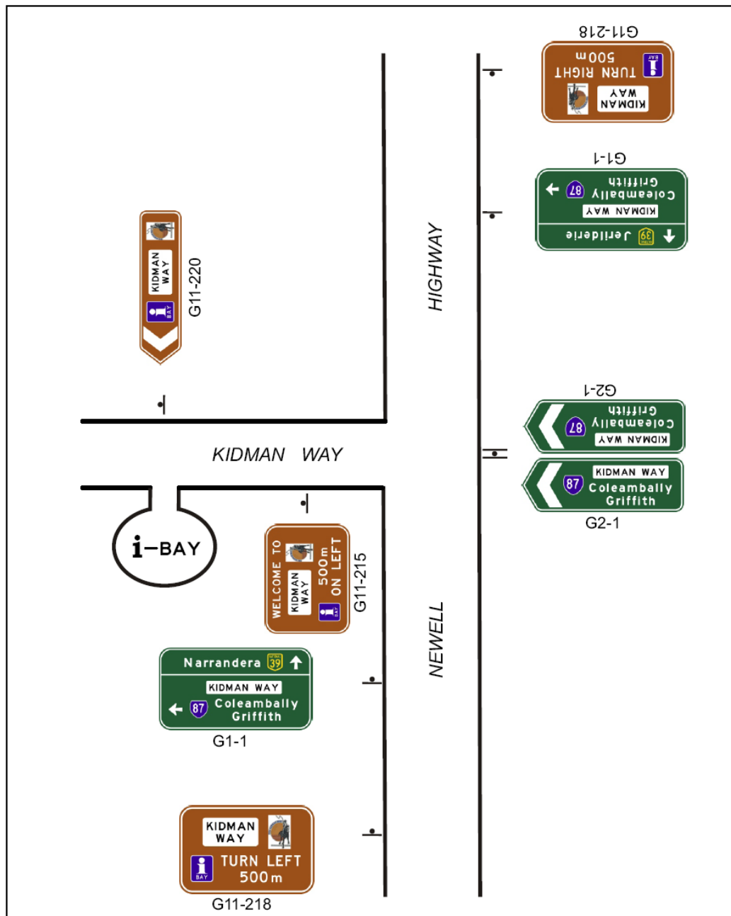
Figure 3.64 Typical arrangement of signs at the start of a touring route where the touring route name is the gazetted road name
